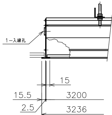
"a"部詳細
